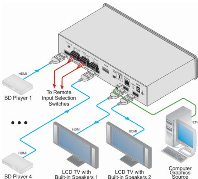
Figure 3: Connecting the VS-42UHD 4x2 HDMI Matrix Switcher
